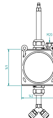
Suspended distributor, plastic with compressed air
