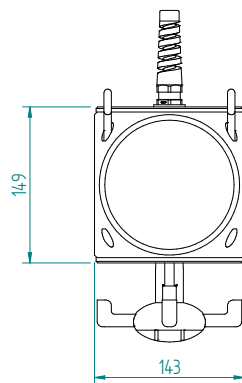
Suspended distributor, plastic
